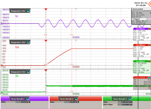
Figure 22 – Output Voltage and Current Waveforms. 85 VAC, 120 mA Output. Upper: V_{IN} , 100 V, 20 ms / div. Middle: V_{OUT} , 2 V / div. Lower: I_{OUT} , 50 mA / div. Rise Time = 34.6 ms.
