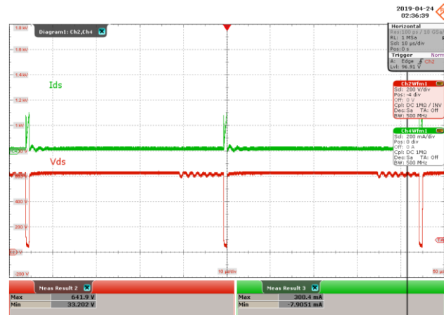
Figure 15 – Drain Voltage and Current Waveforms. 440 VAC, 120 mA Output. Upper: I DRAIN , 200 mA / div. Lower: V DRAIN , 200 V, 10 μs / div. I MAX = 300.4 mA, V MAX = 641.9 V.
