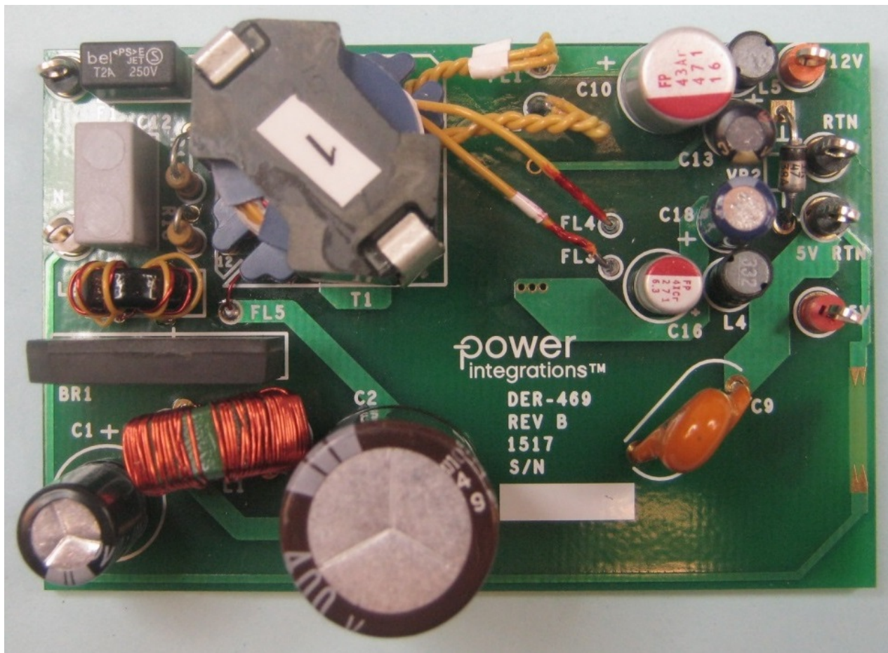
Figure 1 – Populated Circuit Board Photograph, Top.
