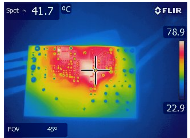
Figure 27 – InnoSwitch-CH Side. 265 VAC, 4 A Load.
