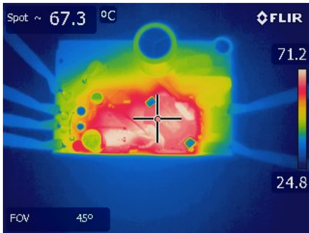
Figure 26 – Transformer Side. 265 VAC, 4 A Load.
