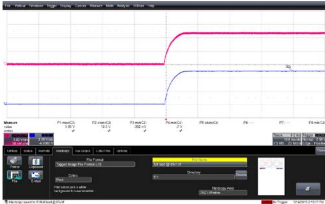
Figure 36 – Output Voltage and Current Waveforms. 85 VAC Input. Upper: 5 V, 2 V / div. Middle: I_{OUT} , 1 A / div. Lower: 12 V, 5 V, 1.6 ms / div.
