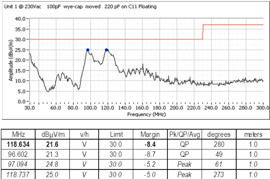
Figure 59 – Floating Ground at 230 VAC.
