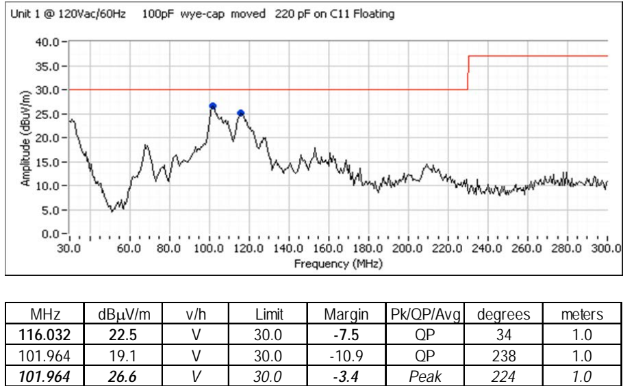
Figure 58 – Floating Ground at 110 VAC.
